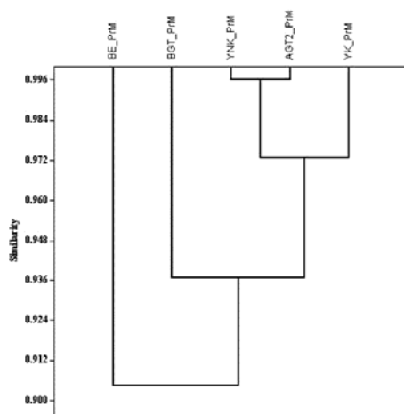
Fig. 4. Cluster analysis of physico-chemical parameters of different streams in Aghanashini river basin of Central Western Ghats during a) monsoon season, (b) post-monsoon and (c) pre-monsoon season.
